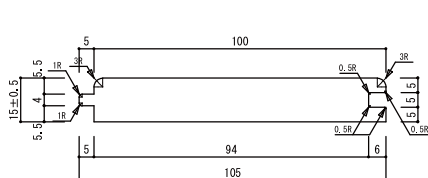
15×100×3,000 (本実)
